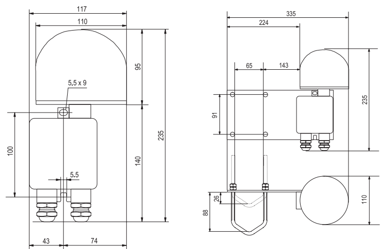
CEL-10-12-F dimensions
