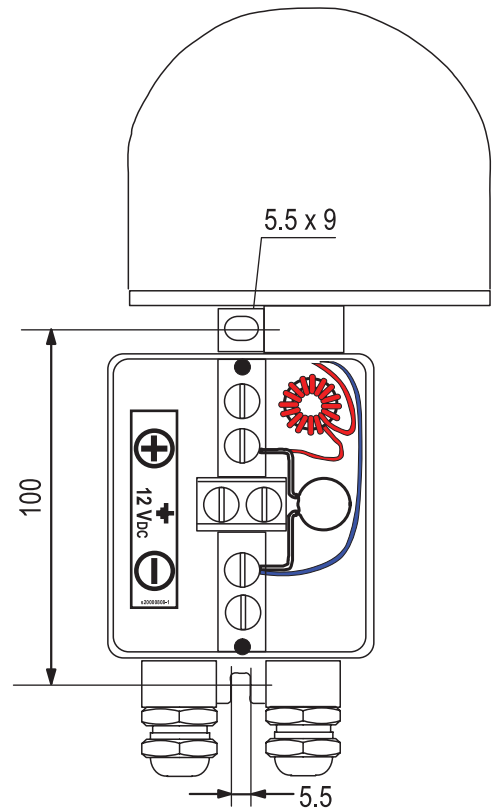
CEL-10-12-F terminal box
