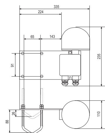
CEL-MS-60 Mounting Set dimensions
